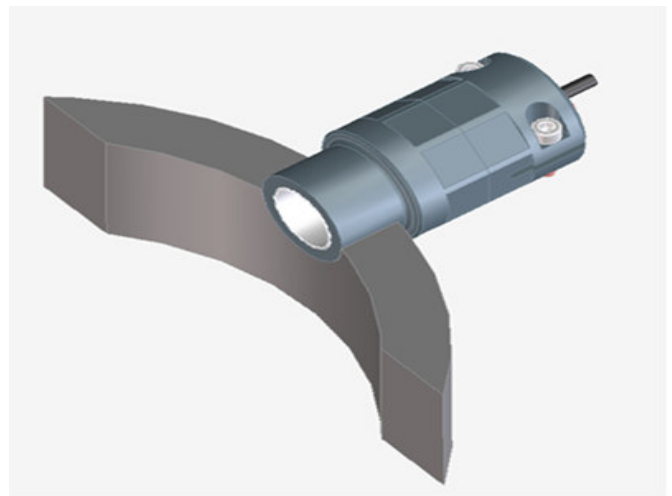
Connection for pipes and for tanks with a wall thickness up to 25 mm
